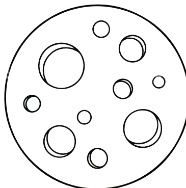
Mercury
