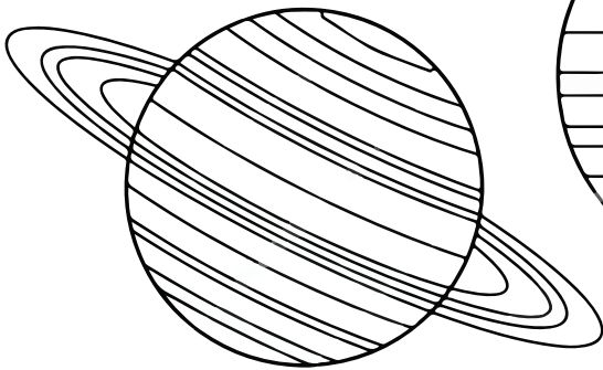
Saturn
